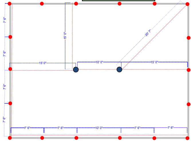
30' x 40' Pole Tent Standard - Pole placement
